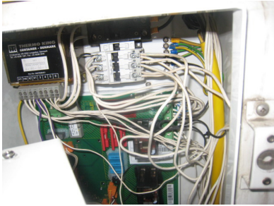
Evap.fans connected parallel with compressor
